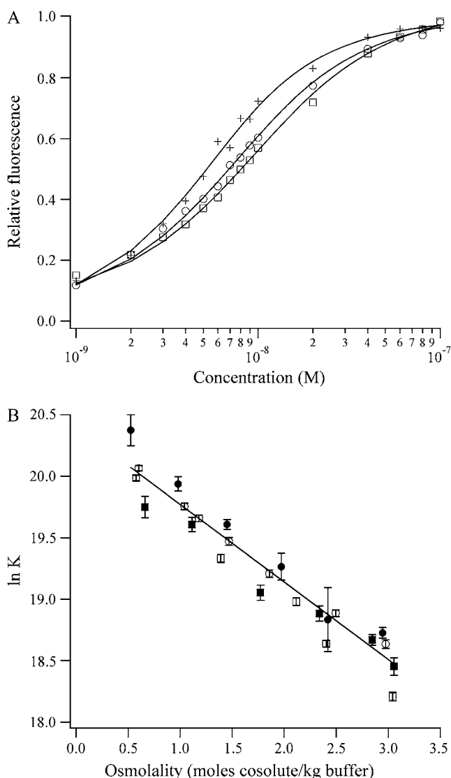
FIGURE 2 (A) Binding isotherms for the titration of the DNA into 10 nM DAPI in buffers with 0.5 M (crosses), 1.5 M (open circles), and 2.5 M (open squares) triethylene glycol show that the affinity of DAPI for the (AATT) 2 binding site decreases with increasing concentrations of triethylene glycol. (B) Plot of the natural logarithm of the observed equilibrium constant for the association of DAPI with the DNA as a function of the concentrations of acetamide (open circles), betaine (open squares), triethylene glycol (solid circles), and trimethylamine N-oxide (solid squares). A linear least-squares fit using Eq. 5 gives 35 \pm 1 waters that are acquired by the complex. The extrapolation to the buffer conditions gives 6.7 (\pm 0.1) \times 10^8 \text{ M}^{-1} .
